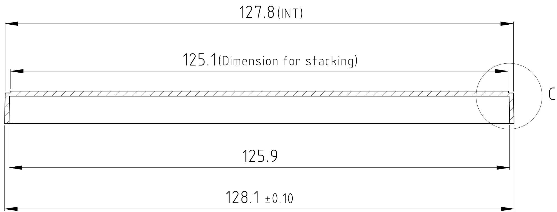
SECTION B-B
