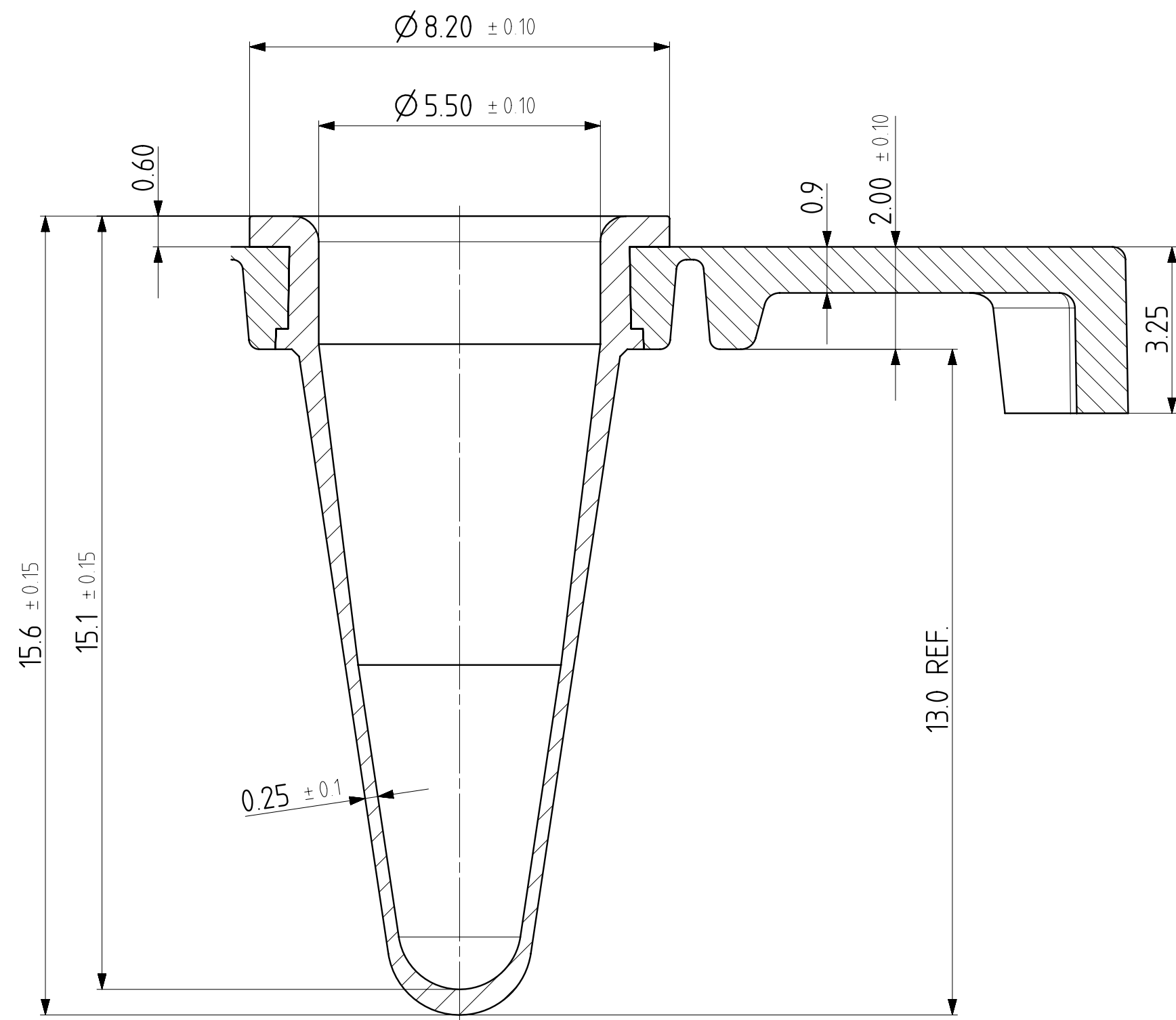
DETAIL B SCALE 10:1
